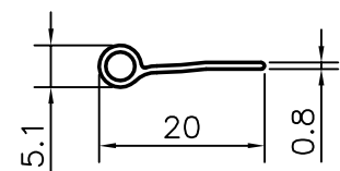
BEADING SECTION
