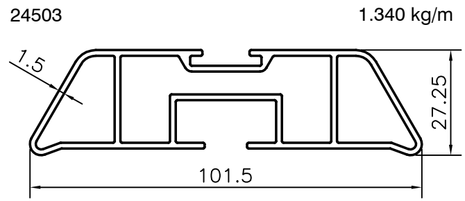
TRANSPORT SECTION
