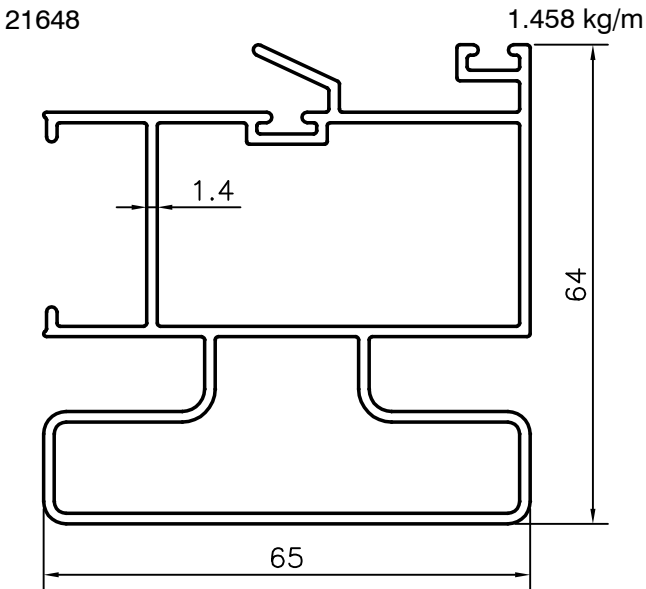
WINDOW SECTION
