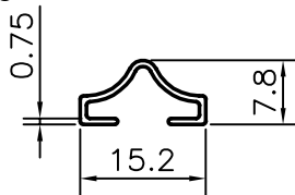
BEADING SECTION
