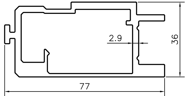
TEXTILE SECTION
