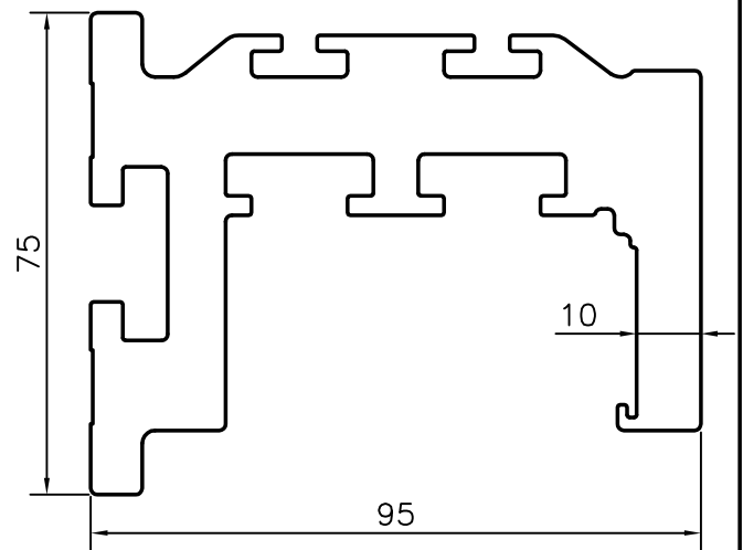
INDUSTRIAL SECTION
