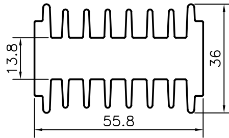
HEAT SINK SECTION
