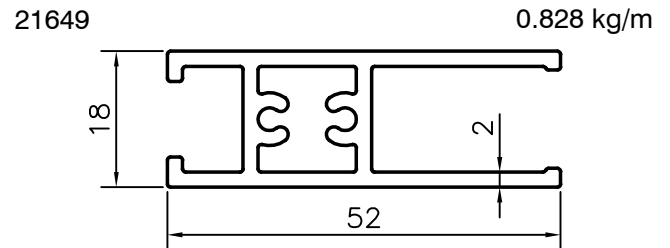
WINDOW SECTION
