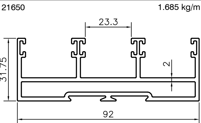
WINDOW SECTION
