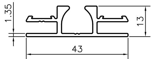
INDUSTRIAL SECTION
