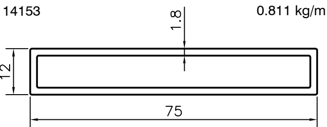
RECTANGULAR TUBE
