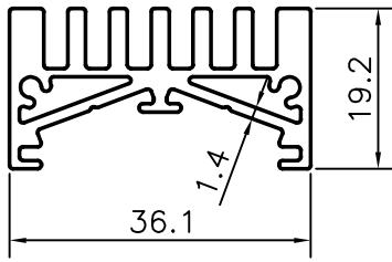
HEAT SINK SECTION
