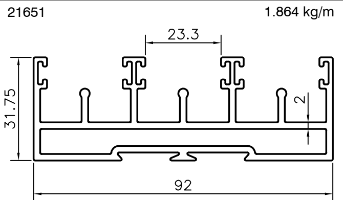
WINDOW SECTION
