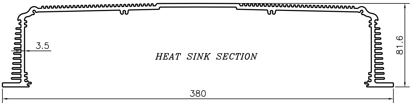
HEAT SINK SECTION
