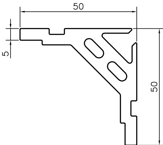
INDUSTRIAL SECTION
