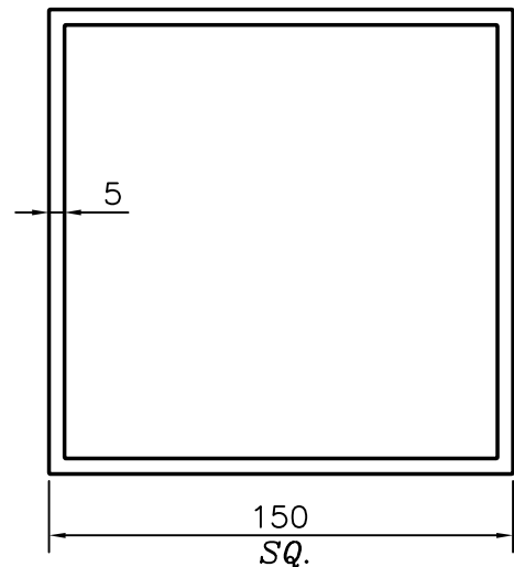
SQUARE TUBE
