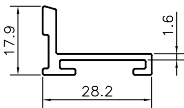
INDUSTRIAL SECTION
