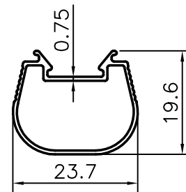
TUBE LIGHT SECTION
