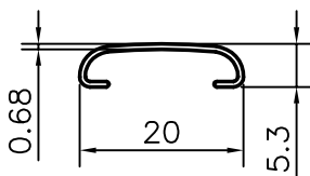
BEADING SECTION
