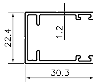
VENETIAN BLIND SECTION
